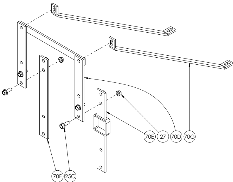
ROLLER MOUNTING BRACKET (PRESSED FRAME & ROLL FORM FRAME) (ITEM 69A FOR "B/B2" ROLLER COMPLETE BRACKET ASSEMBLY) (ITEM 69B FOR "C/C2" ROLLER COMPLETE BRACKET ASSEMBLY)
