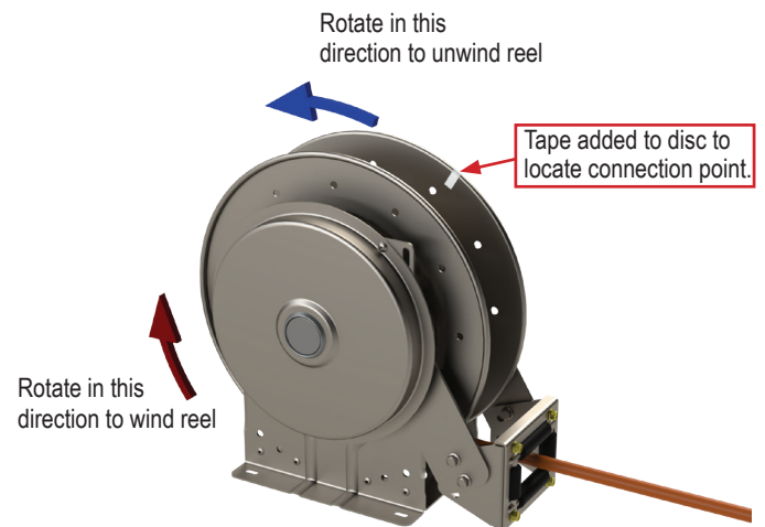
Figure 3 - Reel with Hose Attached Showing Rotation Direction
